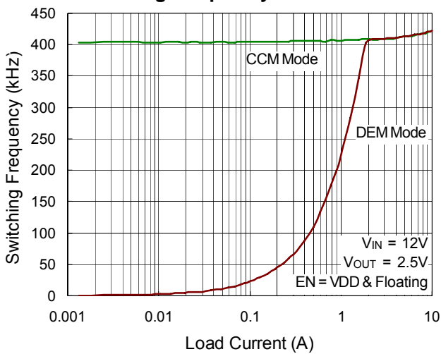
2.5V Switching Frequency vs. Load Current
